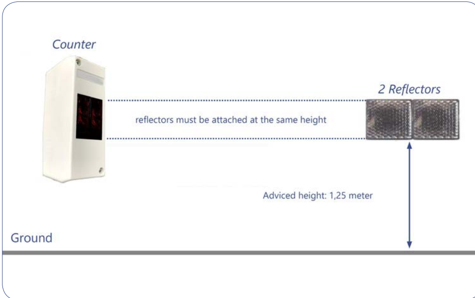
Mounting the counter and reflectors
